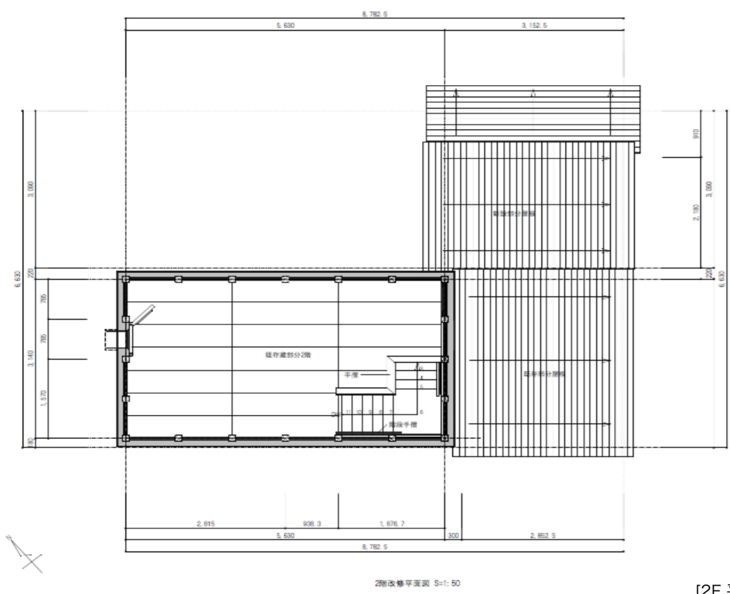
[2F 平面図]
